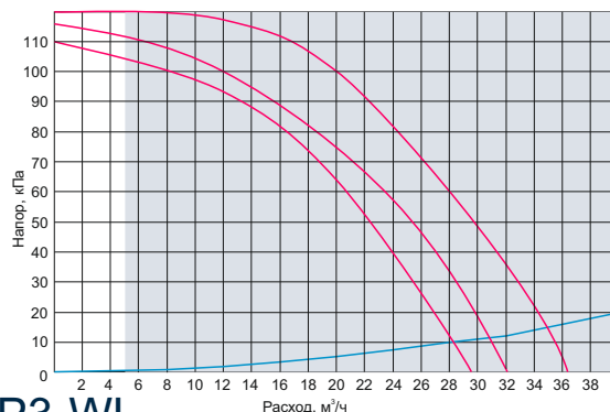
OD-90.0-80-120-P3-WL
