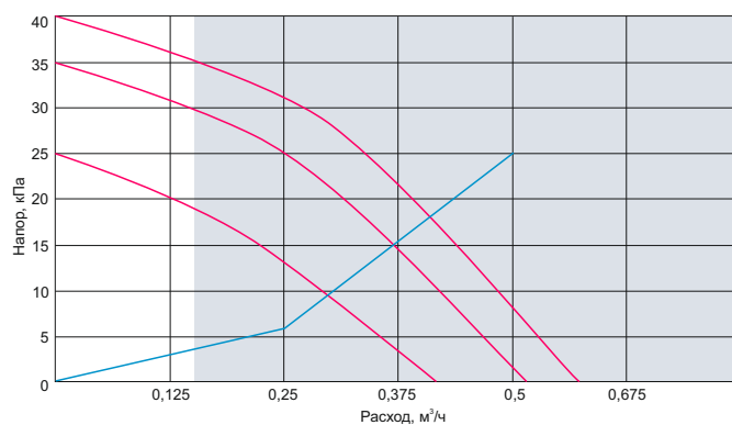
OD-2.5-20-40-P1-WL
